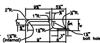
END VIEW CURB CASTING
