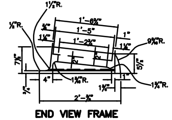
END VIEW FRAME
