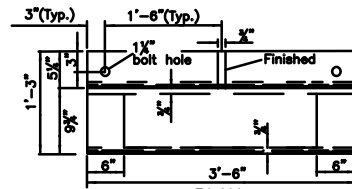
PLAN CURB CASTING
