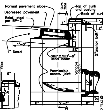
SECTION B-B WITH CURB & GUTTER
