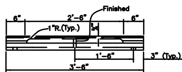
FRONT VIEW CURB CASTING
