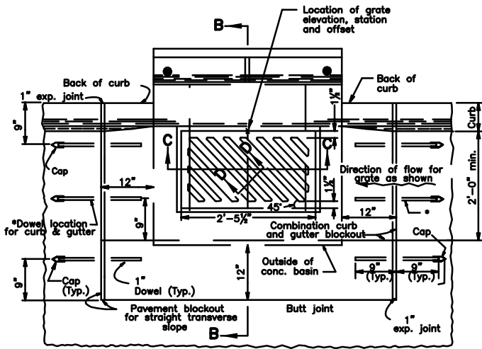
PLAN OF CATCH BASIN AND PAVEMENT JOINTS
